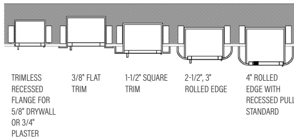
ADA COMPLIANT CABINET STYLES - TOP VIEW
