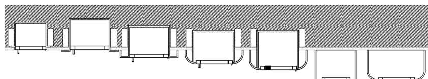
TRIMLESS RECESSED FLANGE FOR 5/8" DRYWALL OR 3/4" PLASTER
