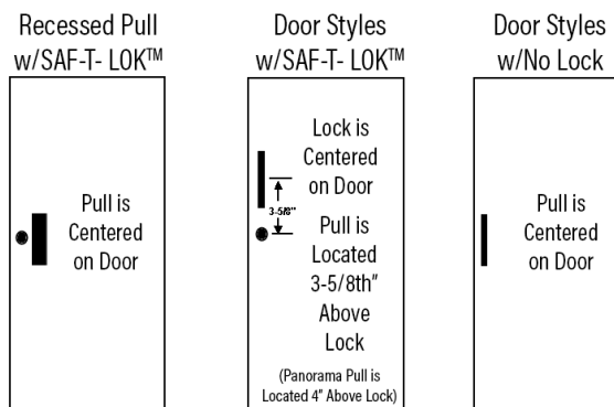
ADA MOUNTING HEIGHTS
